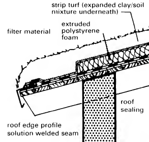
⑪ Detail of the eaves on a sloping 'green' roof
